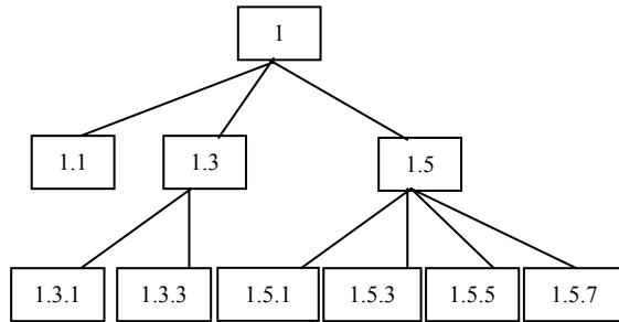
Figure 1: ORDPATH scheme
